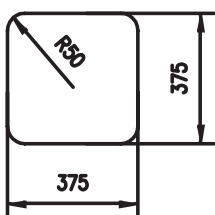
Material: Stahl/Steel
