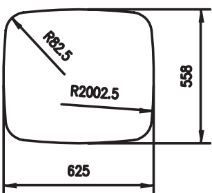
Material: Aluminium Querschnitt/Cross section: 824
